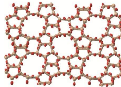
a) Silicalite (MFI framework)
